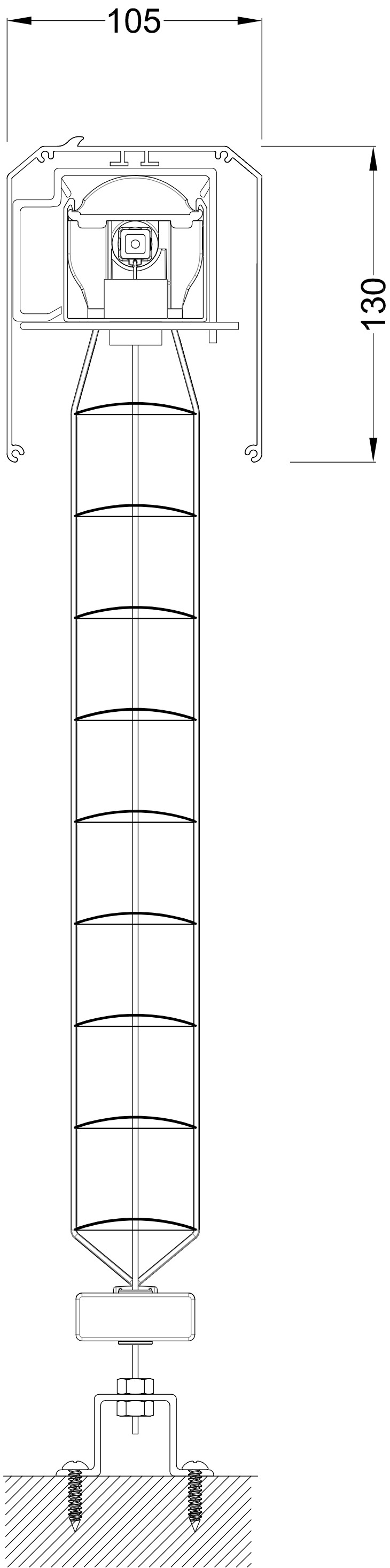
FLOOR MOUNT
